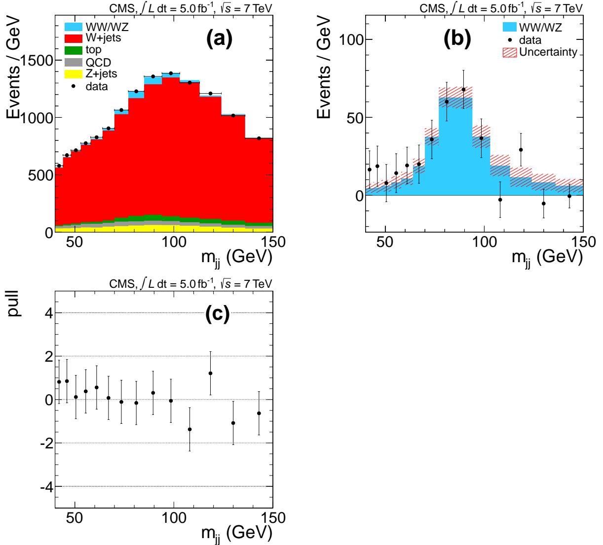
Figure 1: (a) Distribution of the dijet invariant mass in data, with the binning chosen based on the resolution and fit projections of the relevant components overlaid. (b) The dijet invariant mass after subtraction of all components except the electroweak WW+WZ processes. The error bars represent the statistical uncertainties and the hatched bands represent the systematic uncertainties. (c) The normalized residual or pull: (\text{data} - \text{fit}) / (\text{fit uncertainty}) .
