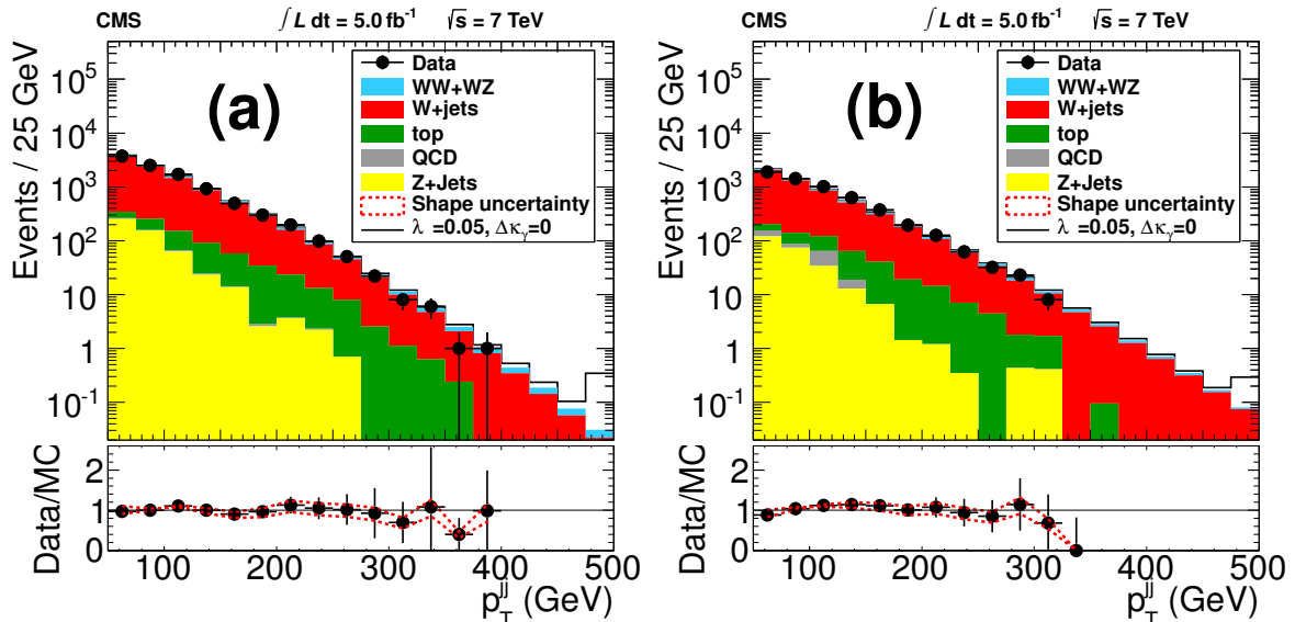
Figure 2: Dijet p_T distributions for (a) the muon and (b) the electron channels after full selection and with the requirement 75 \text{ GeV} < m_{jj} < 95 \text{ GeV} . The stacked histogram shapes are taken from simulation or, where applicable, from data-driven estimates. They are normalized according to the fit to the observed m_{jj} spectrum in data. Below we show the Data/MC ratio with the (dashed) red lines corresponding to the shape uncertainty. The last bin includes the overflow.
