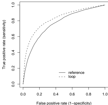
Figure 5: ROC curve for the simulation study: 100 genes, of which 30 are differentially expressed, across 3 conditions using 6 arrays for each design.
