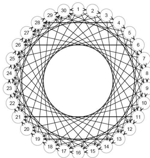
Figure 8: A-optimal design for an experiment with 30 time-points and 90 arrays in the class of interwoven loop designs.
